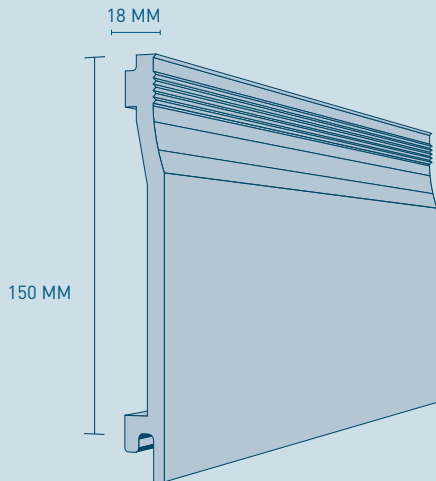
SIDINGS 150 MM
